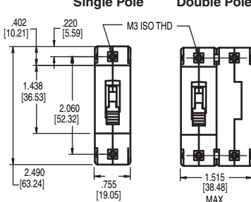
Single Pole Double Pole
